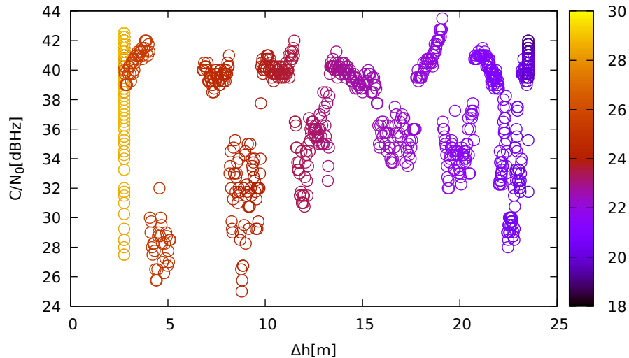
C/N 0 vs height (JavadLSA (up) for G16 at L1)
