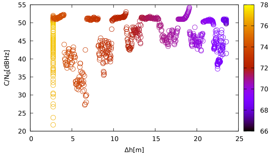
C/N 0 vs height (JavadLSA (up) for G18 at L1)
