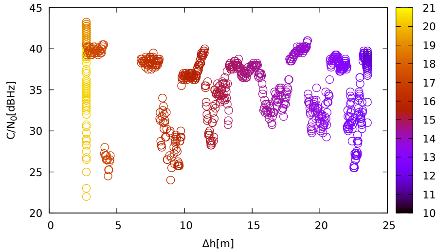
C/N 0 vs height (JavadLSA (up) for G20 at L1)
