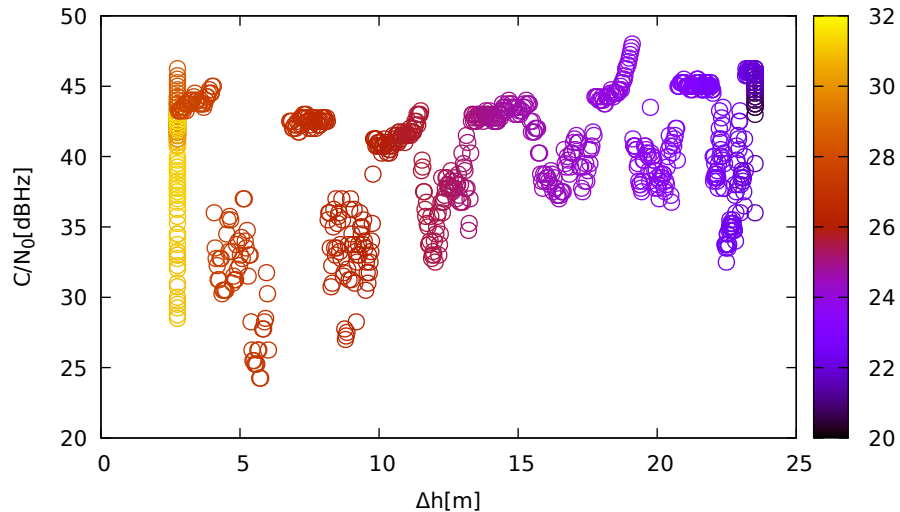
C/N 0 vs height (JavadLSA (up) for G21 at L1)
