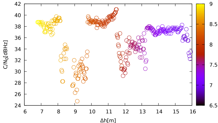
C/N 0 vs height (JavadLSA (up) for G23 at L1)
