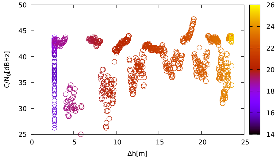
C/N 0 vs height (JavadLSA (up) for G25 at L1)
