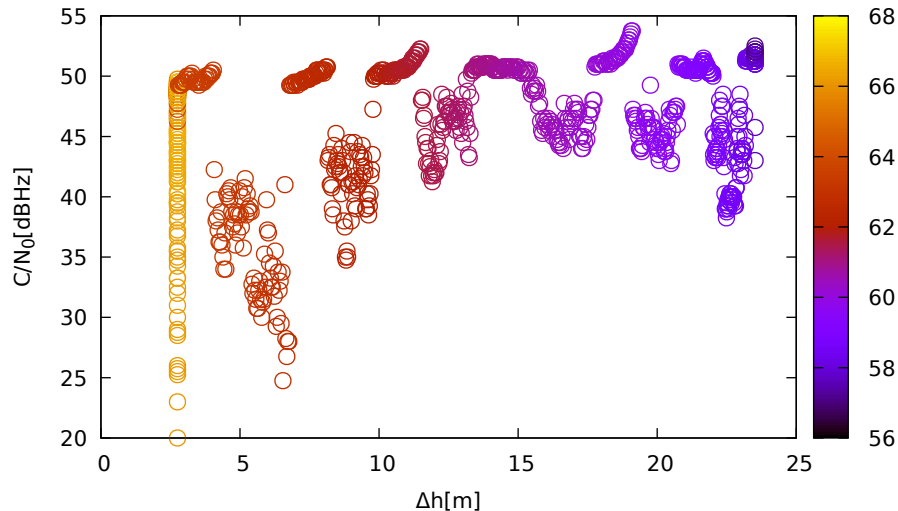
C/N 0 vs height (JavadLSA (up) for G26 at L1)
