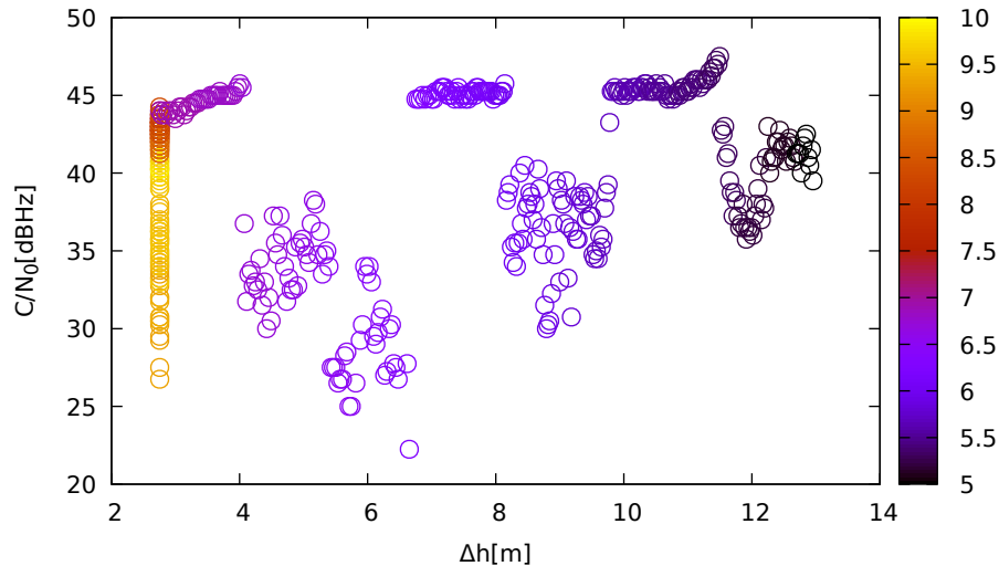
C/N 0 vs height (JavadLSA (up) for G27 at L1)
