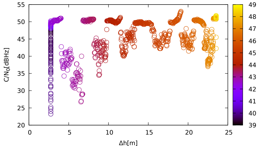
C/N 0 vs height (JavadLSA (up) for G29 at L1)
