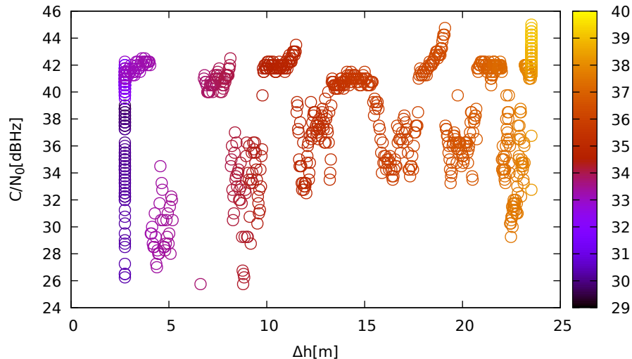
C/N 0 vs height (JavadLSA (up) for G31 at L1)
