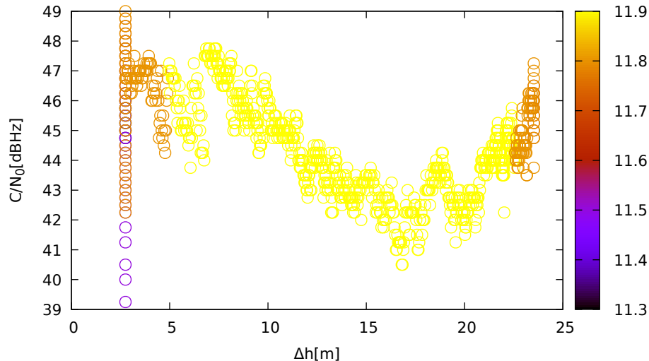
C/N 0 vs height (JavadLSA (up) for R02 at L1)
