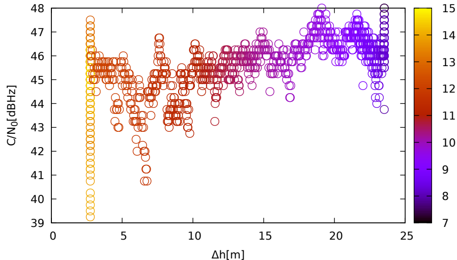
C/N 0 vs height (JavadLSA (up) for R03 at L1)
