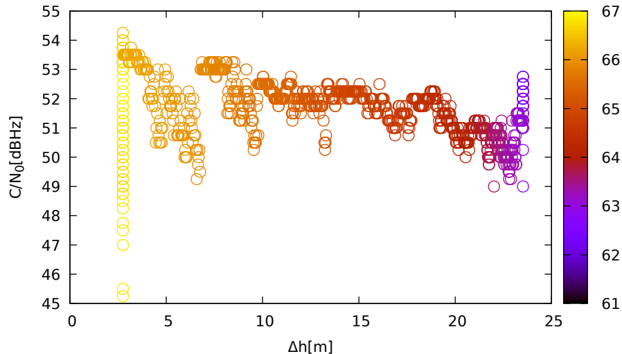
C/N 0 vs height (JavadLSA (up) for R09 at L1)
