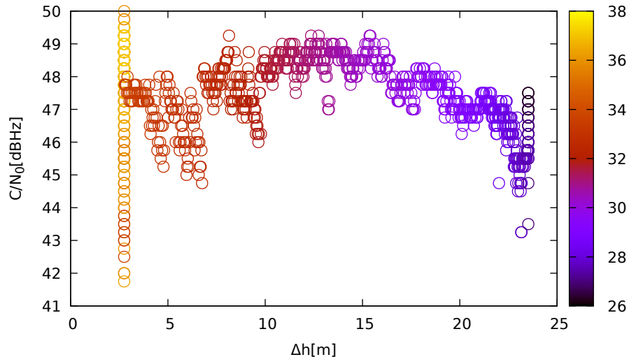
C/N 0 vs height (JavadLSA (up) for R10 at L1)
