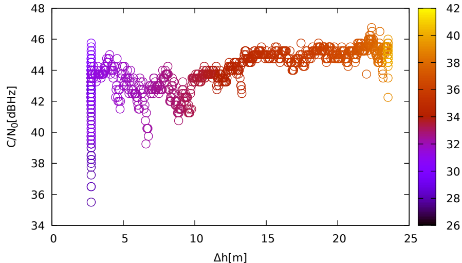
C/N 0 vs height (JavadLSA (up) for R16 at L1)
