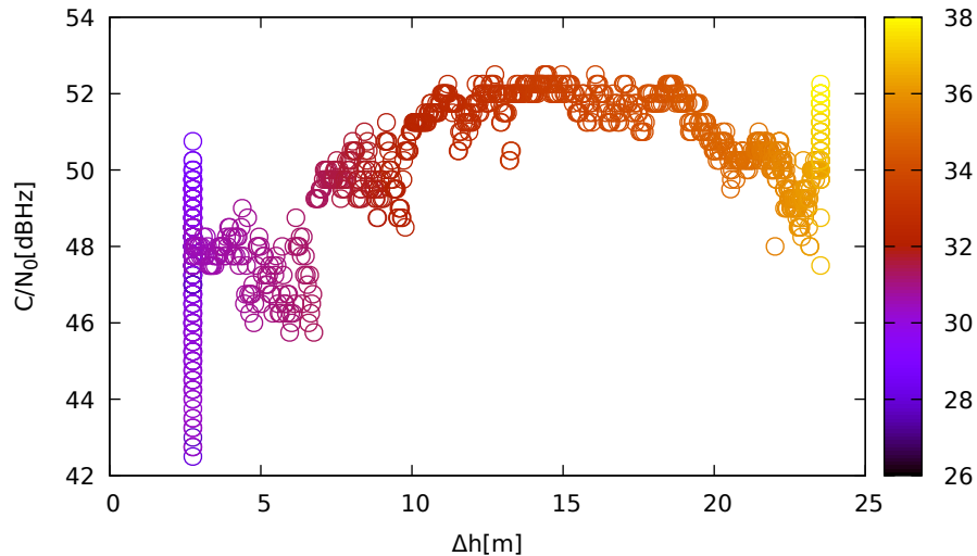
C/N 0 vs height (JavadLSA (up) for R18 at L1)
