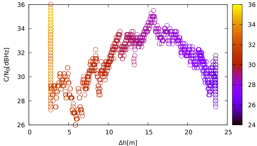
C/N 0 vs height (JavadLSA (up) for R20 at L1)
