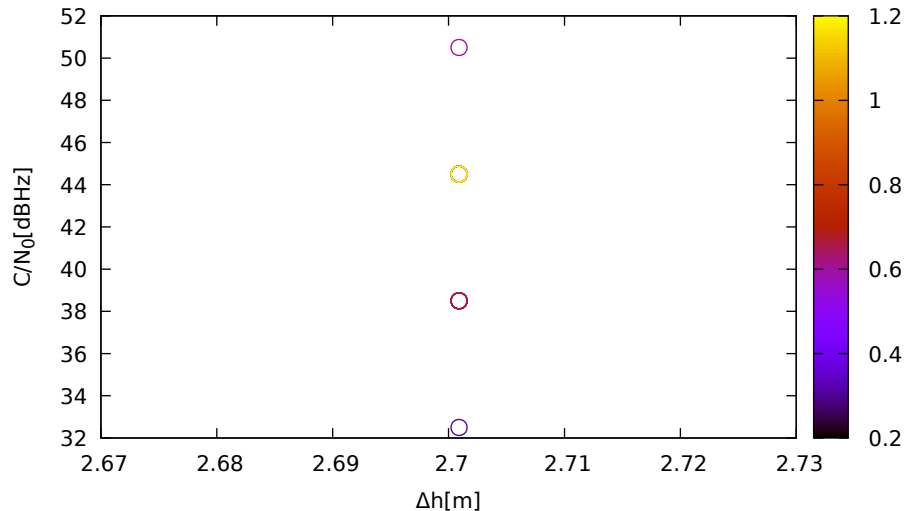
C/N 0 vs height (LeicaGS15 (up) for E07 at L1)
