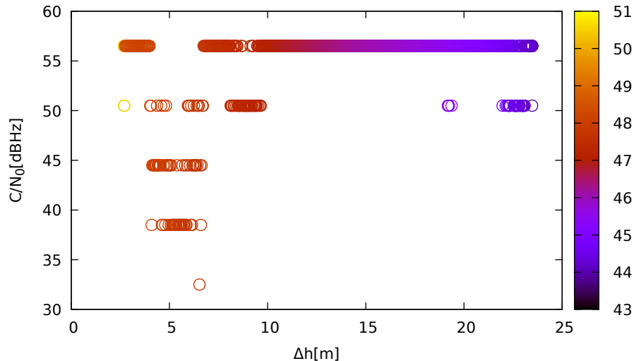
C/N 0 vs height (LeicaGS15 (up) for E24 at L1)
