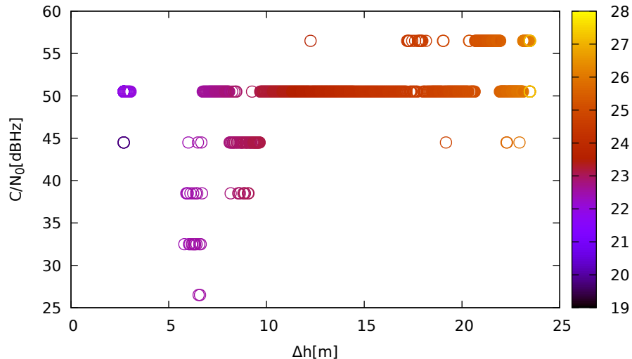
C/N 0 vs height (LeicaGS15 (up) for E26 at L1)
