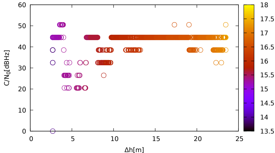
C/N 0 vs height (LeicaGS15 (up) for G05 at L1)
