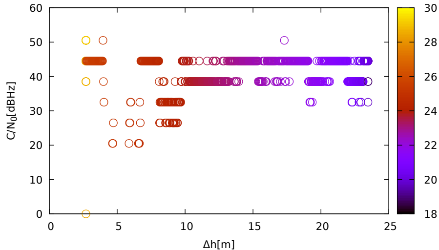
C/N 0 vs height (LeicaGS15 (up) for G16 at L1)
