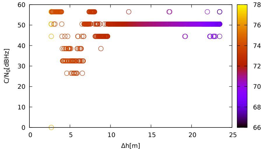
C/N 0 vs height (LeicaGS15 (up) for G18 at L1)
