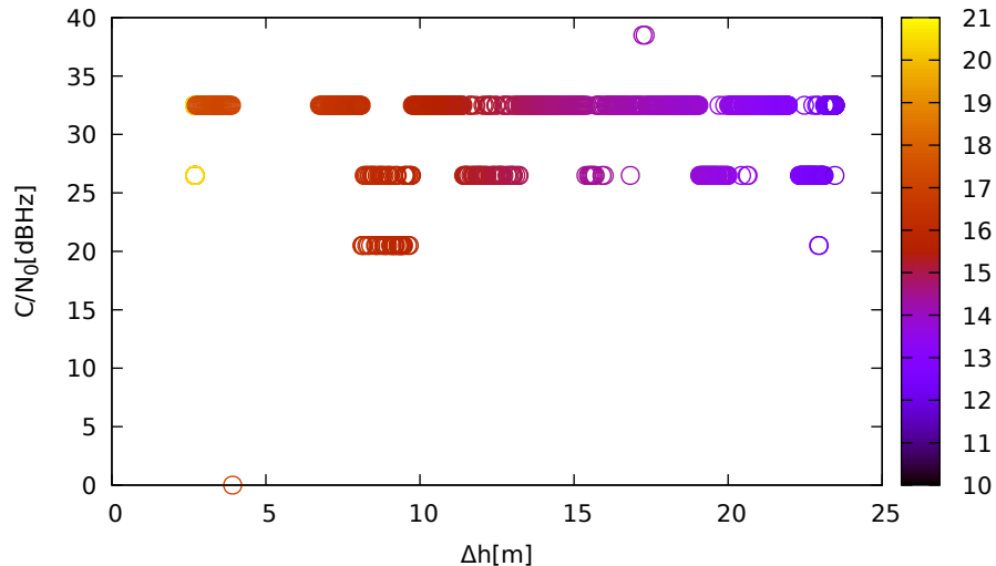
C/N 0 vs height (LeicaGS15 (up) for G20 at L1)
