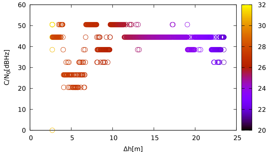
C/N 0 vs height (LeicaGS15 (up) for G21 at L1)
