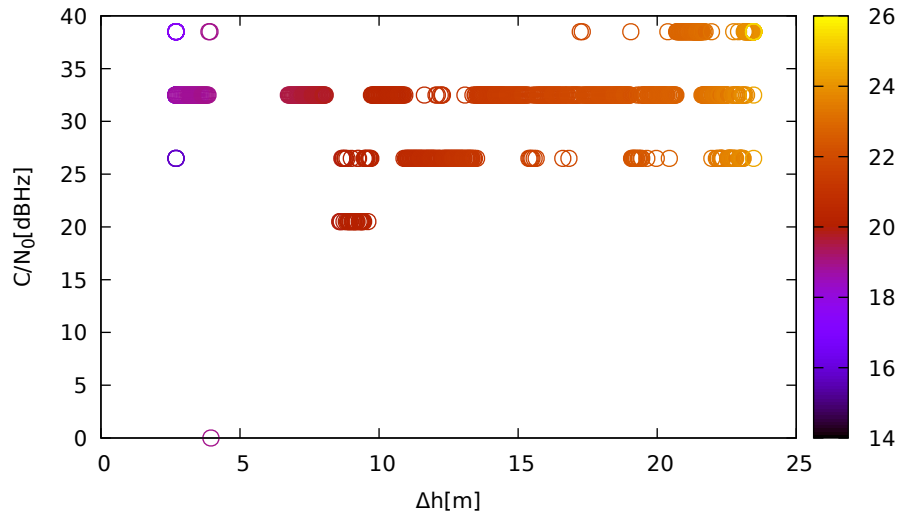
C/N 0 vs height (LeicaGS15 (up) for G25 at L1)
