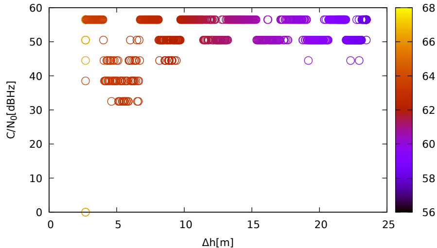
C/N 0 vs height (LeicaGS15 (up) for G26 at L1)
