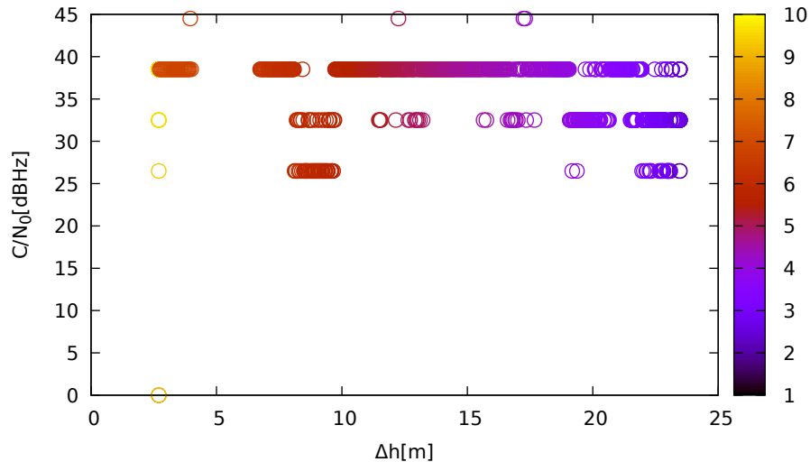
C/N 0 vs height (LeicaGS15 (up) for G27 at L1)
