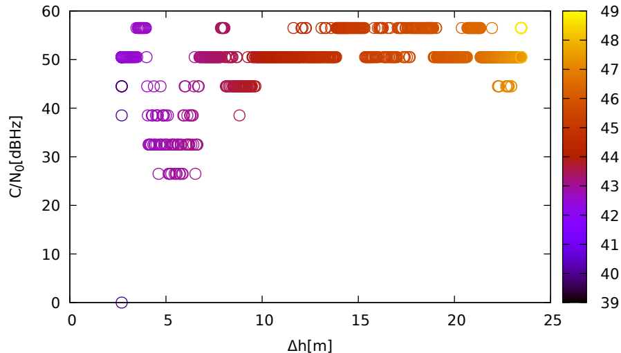
C/N 0 vs height (LeicaGS15 (up) for G29 at L1)
