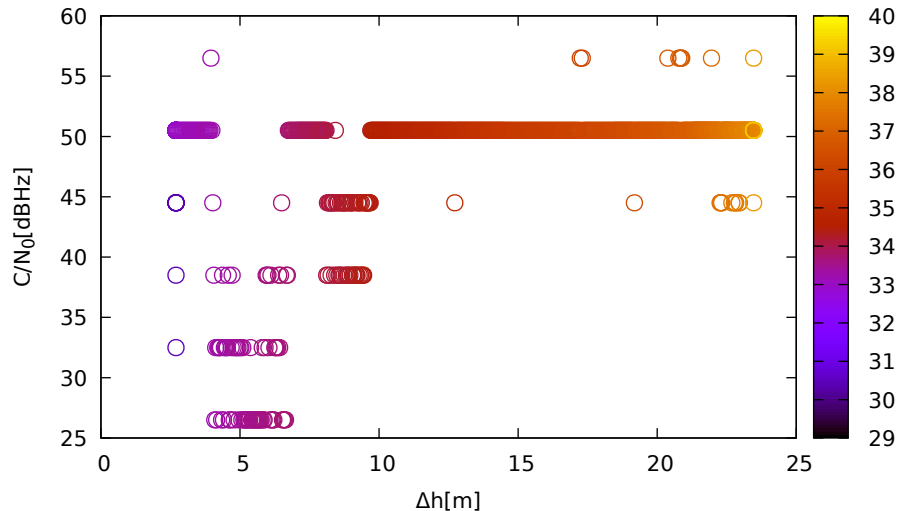
C/N 0 vs height (LeicaGS15 (up) for G31 at L1)
