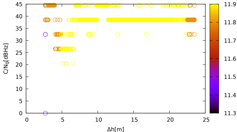
C/N 0 vs height (LeicaGS15 (up) for R02 at L1)
