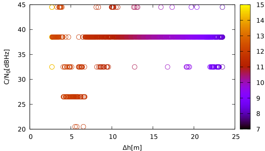
C/N 0 vs height (LeicaGS15 (up) for R03 at L1)
