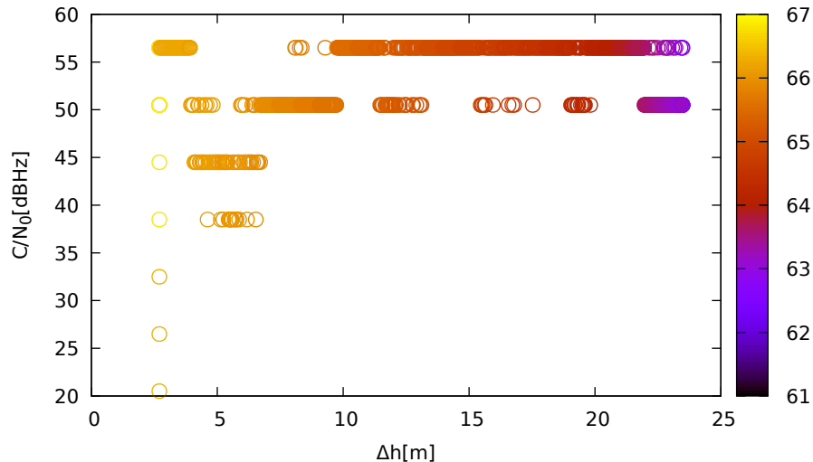
C/N 0 vs height (LeicaGS15 (up) for R09 at L1)
