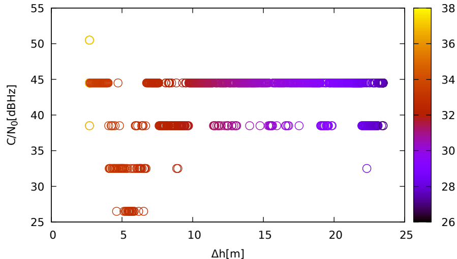
C/N 0 vs height (LeicaGS15 (up) for R10 at L1)
