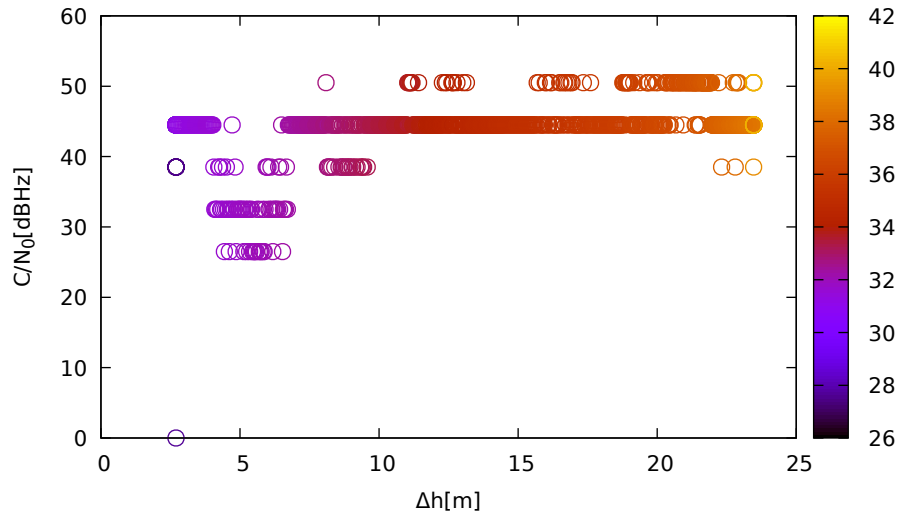
C/N 0 vs height (LeicaGS15 (up) for R16 at L1)
