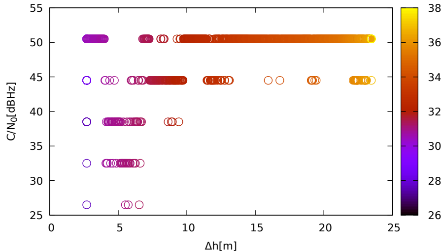
C/N 0 vs height (LeicaGS15 (up) for R18 at L1)
