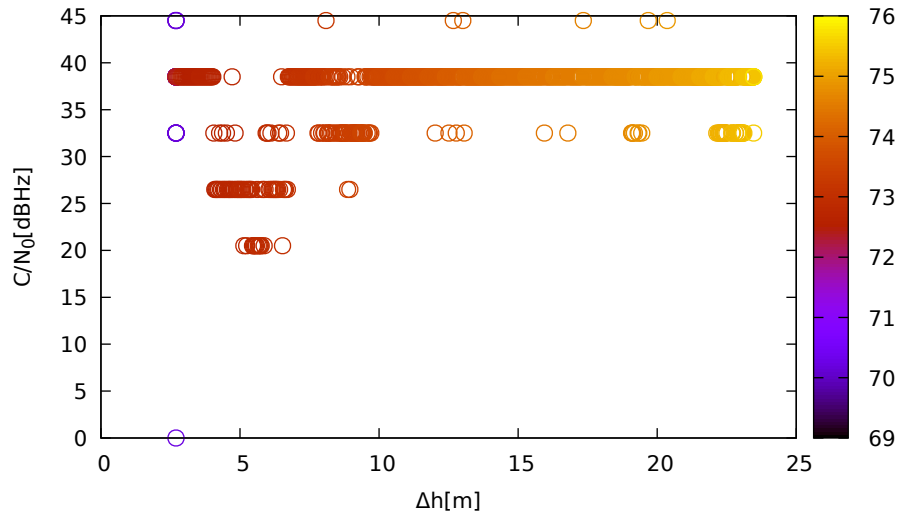
C/N 0 vs height (LeicaGS15 (up) for R19 at L1)
