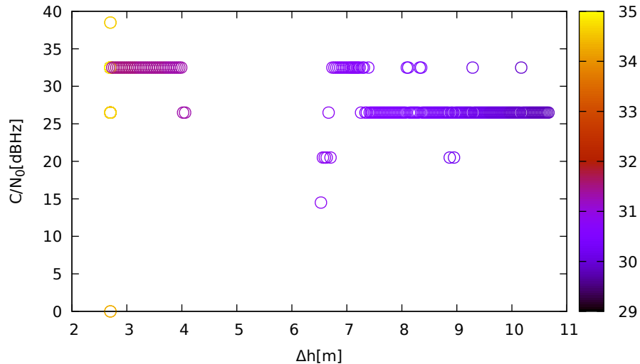
C/N 0 vs height (LeicaGS15 (up) for R20 at L1)
