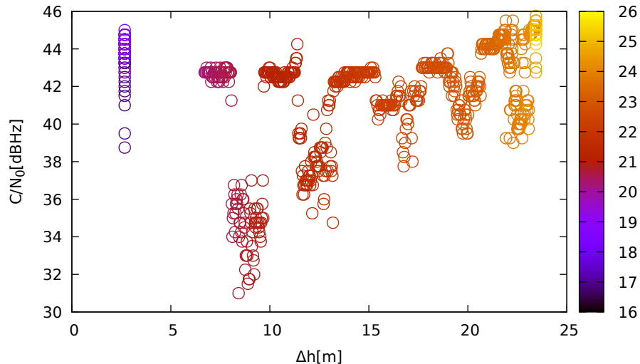
C/N 0 vs height (LeicaGS18 (up) for E01 at L1)
