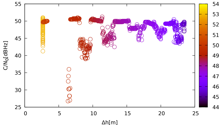
C/N 0 vs height (LeicaGS18 (up) for E12 at L1)
