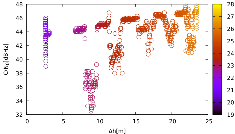
C/N 0 vs height (LeicaGS18 (up) for E26 at L1)
