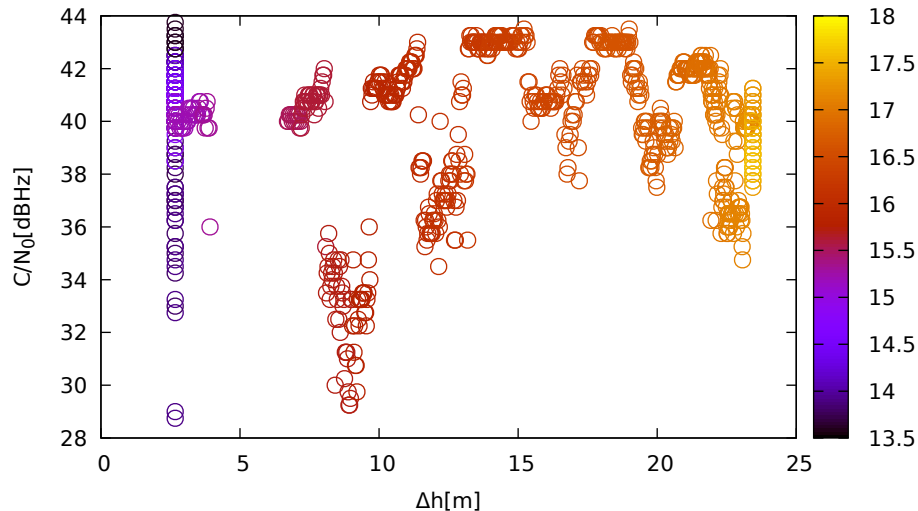
C/N 0 vs height (LeicaGS18 (up) for G05 at L1)
