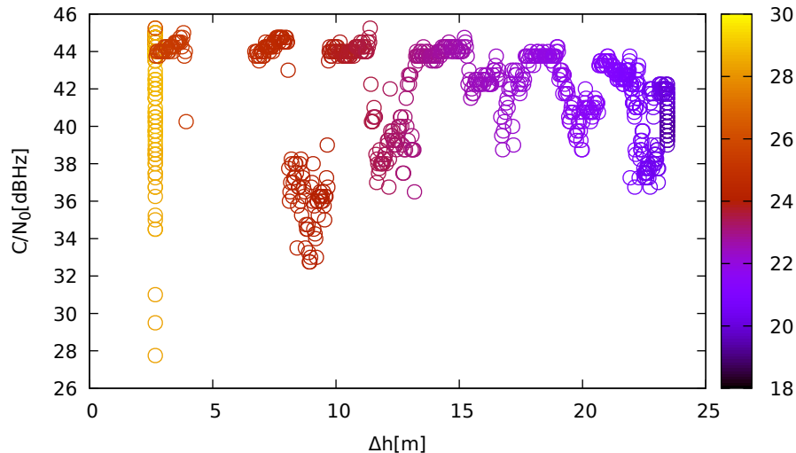
C/N 0 vs height (LeicaGS18 (up) for G16 at L1)
