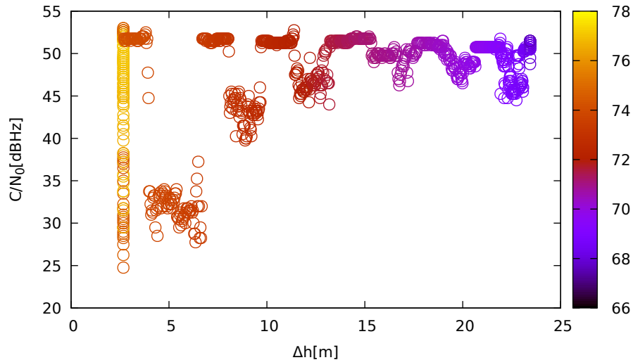
C/N 0 vs height (LeicaGS18 (up) for G18 at L1)
