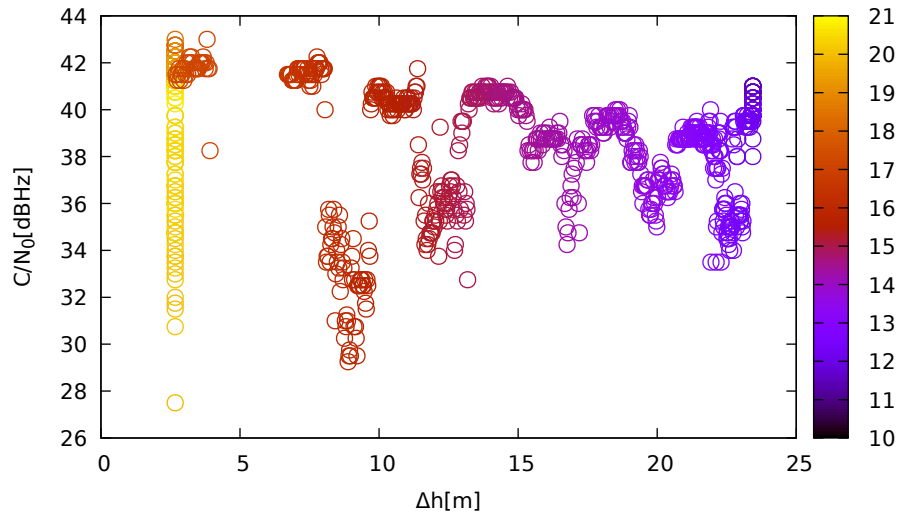
C/N 0 vs height (LeicaGS18 (up) for G20 at L1)
