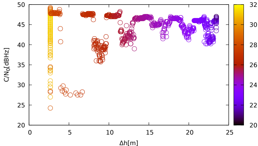
C/N 0 vs height (LeicaGS18 (up) for G21 at L1)
