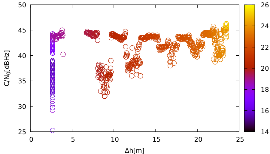
C/N 0 vs height (LeicaGS18 (up) for G25 at L1)
