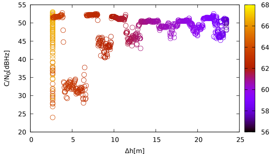
C/N 0 vs height (LeicaGS18 (up) for G26 at L1)
