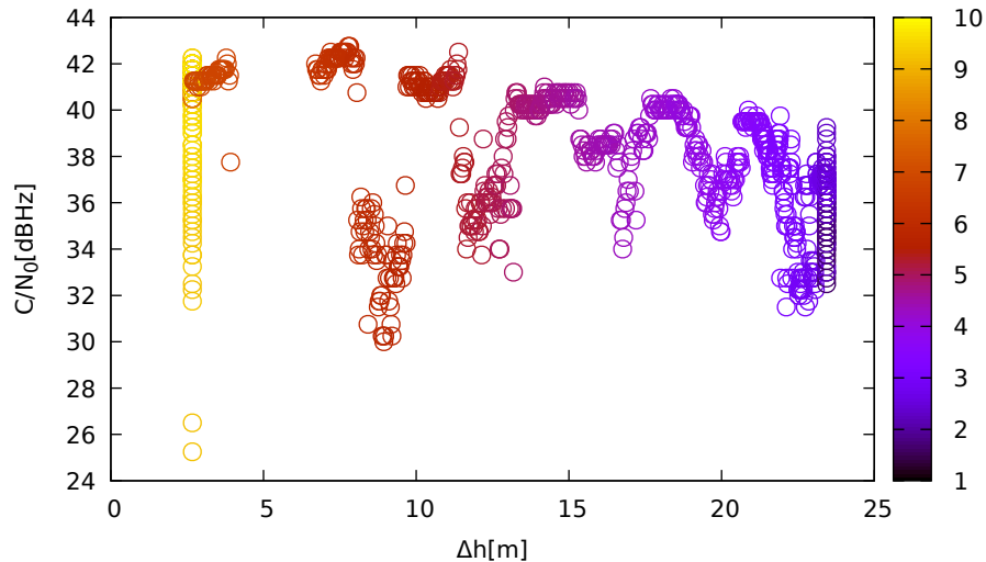
C/N 0 vs height (LeicaGS18 (up) for G27 at L1)
