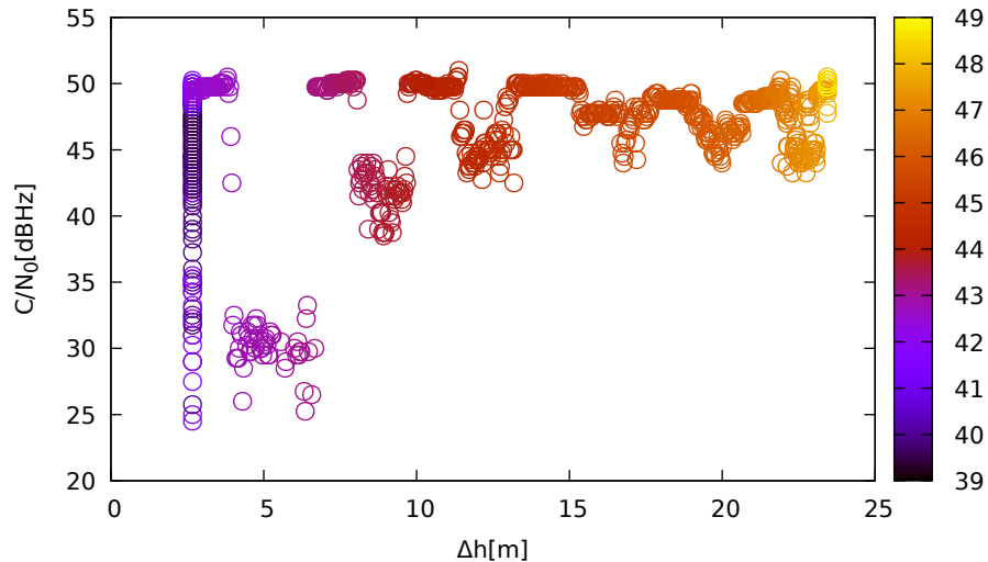
C/N 0 vs height (LeicaGS18 (up) for G29 at L1)
